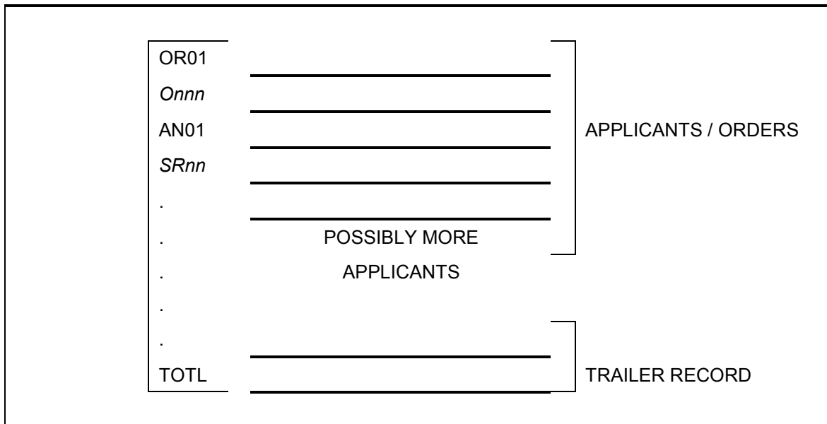
Figure 1: File Representation
